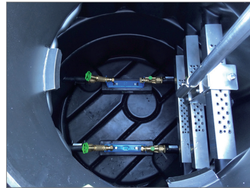
Water meter chamber with integrated installation fittings
