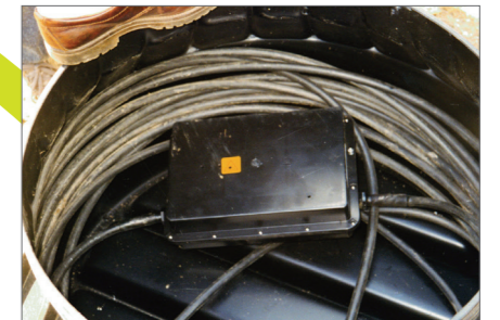
Watertight – good cable positioning and installation options
