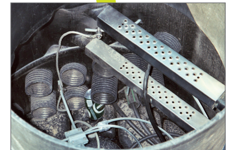
Climbing steps can be easily removed if necessary (cable installation).
