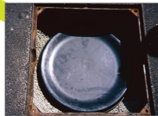
Watertight chamber cover system with separate sealing and load-bearing function
